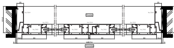
HORIZONTAL SECTION DETAIL
