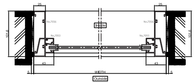
HORIZONTAL SECTION DETAIL
